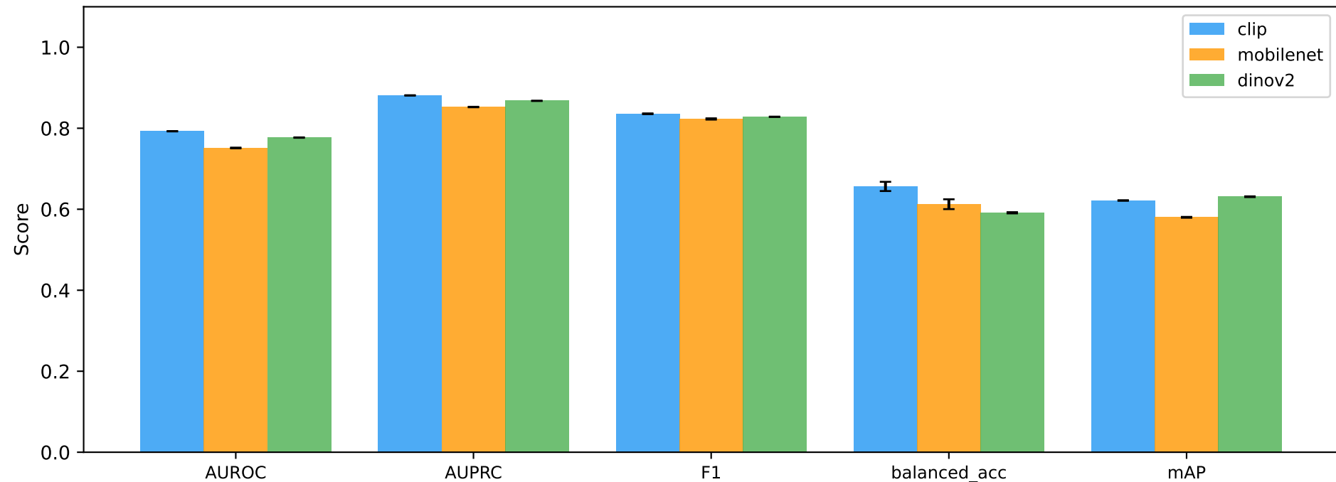
Backbone Comparison - Triage + Defect (mean \pm std, 5 seeds)
